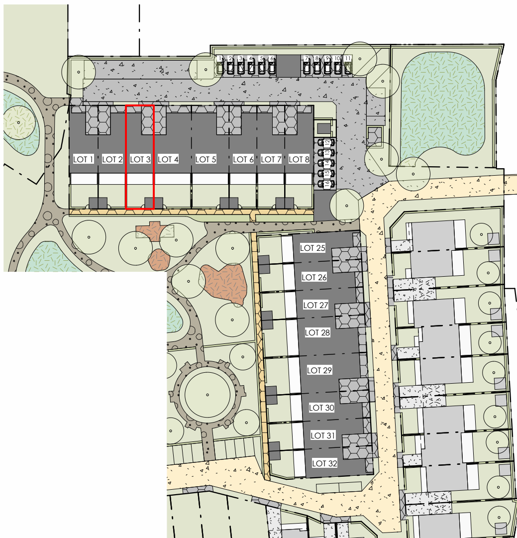
INPLANTINGSPLAN 1:1000
